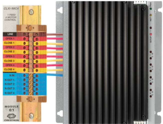
CLXI-1MC4 SHOWN WITH CLTI-1MC4 TERMINATION BLOCK
