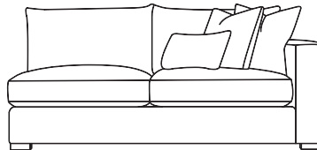
RIGHT ARM LOVESEAT N5241 W 80.50 | D 40 | H 32.50 in. SH 17.50 | AH 26.50 | SD 26.50 in.
