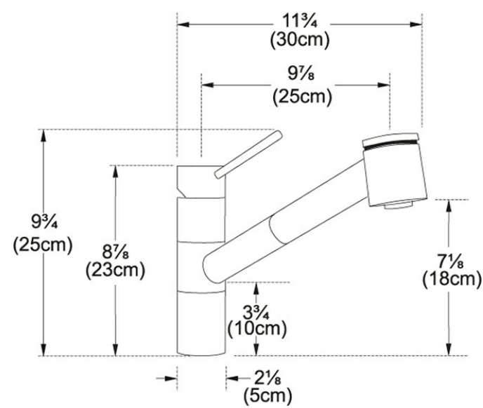
Technical Drawing
