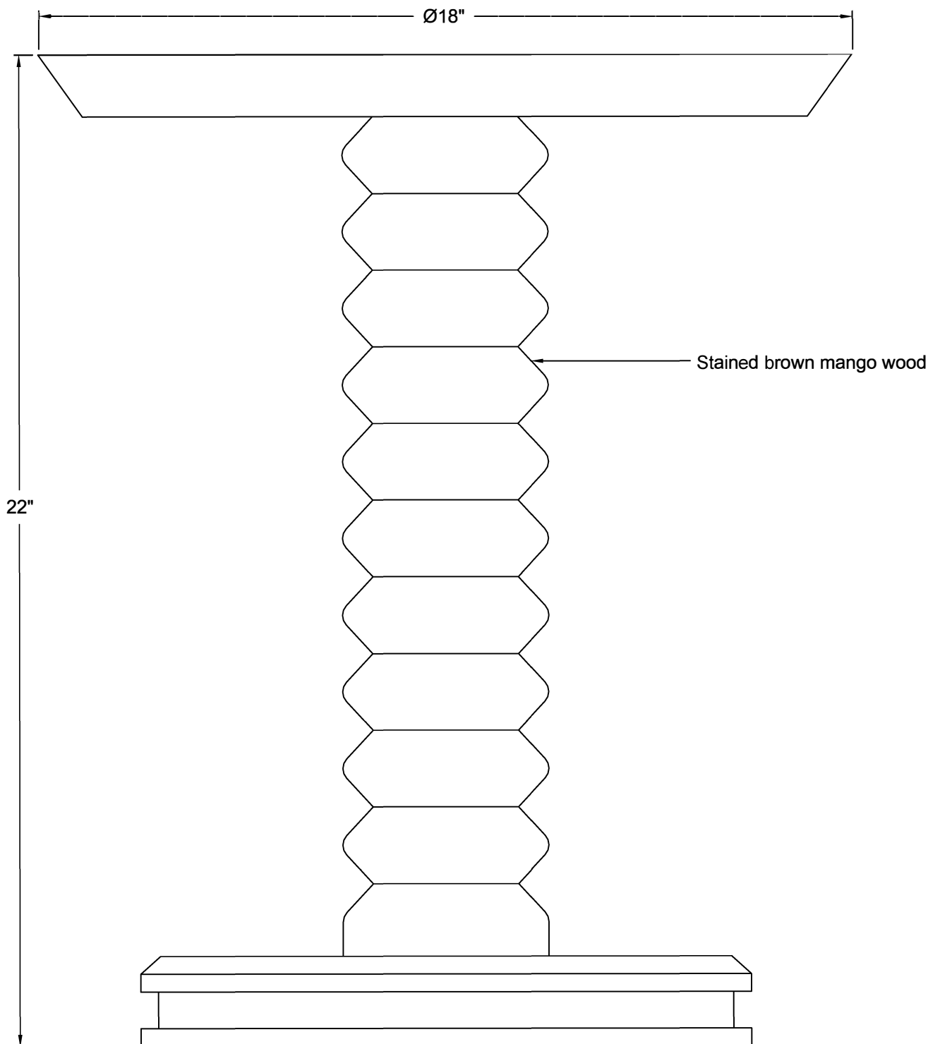
FRONT VIEW
