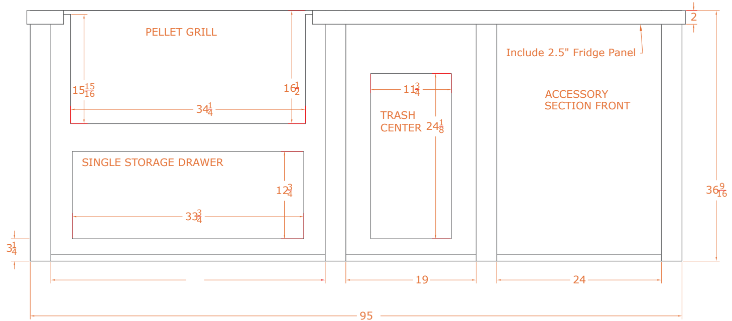
FRONT VIEW
