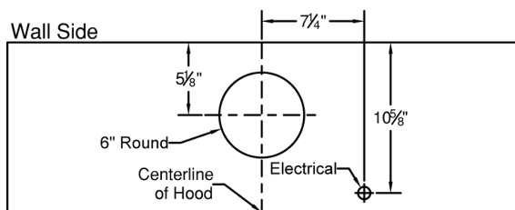
M600 & M1200 Connection Diagrams
