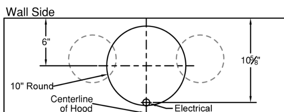
M600 & M1200 Connection Diagrams
