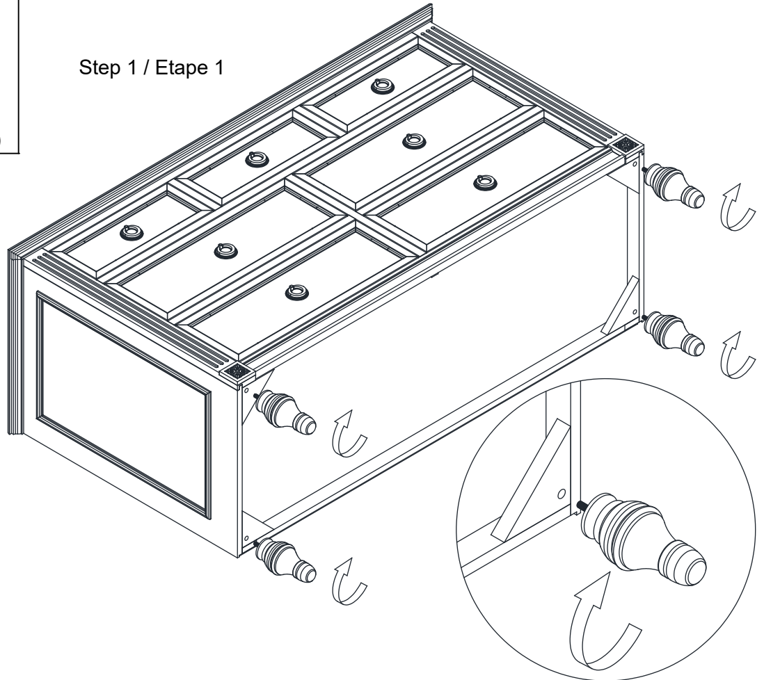
Removable Feet / Pieds amovibles ( x4 )
