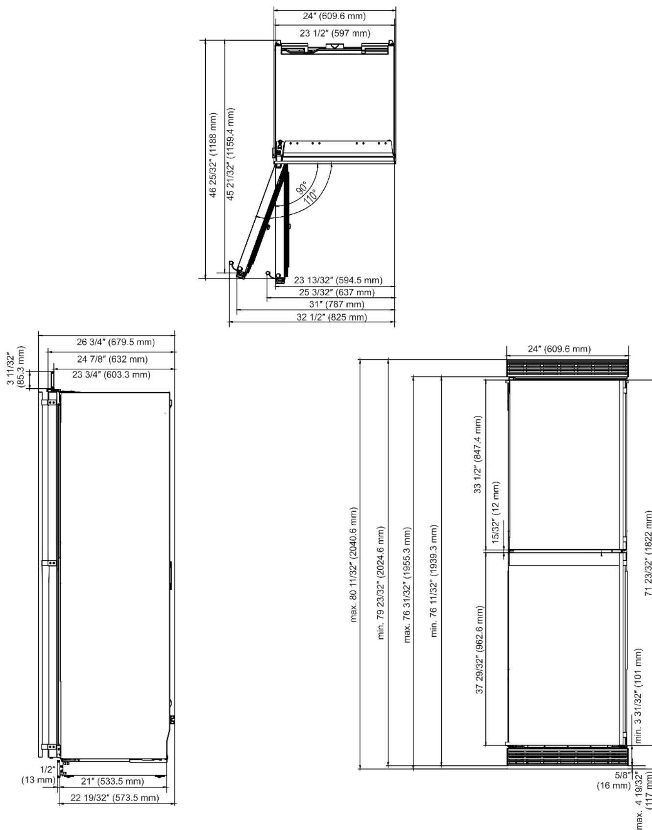
Fig. 1 Single-unit installation
