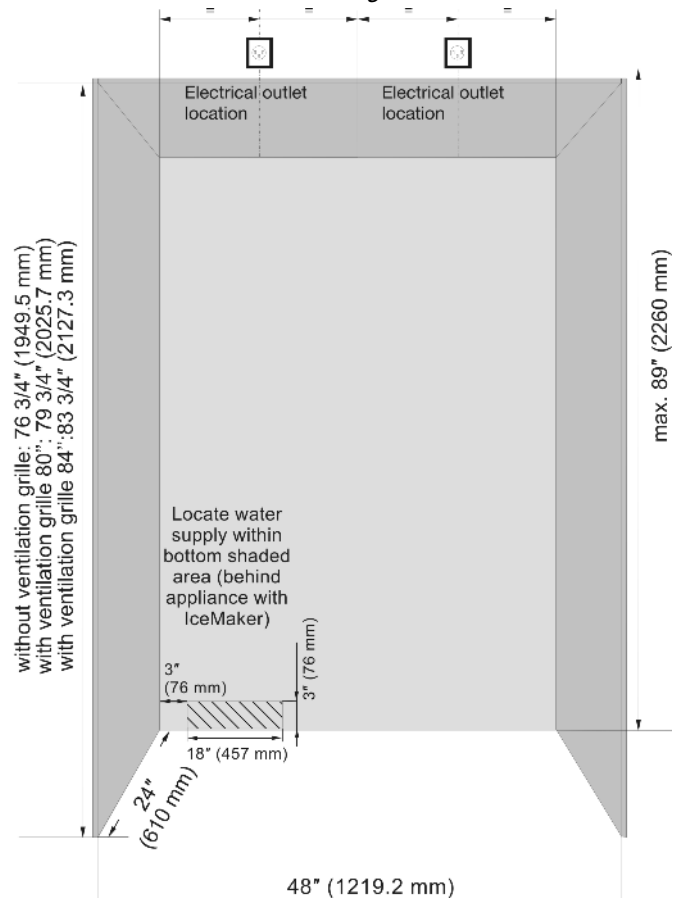
Fig. 6 Side-by-side installation:
