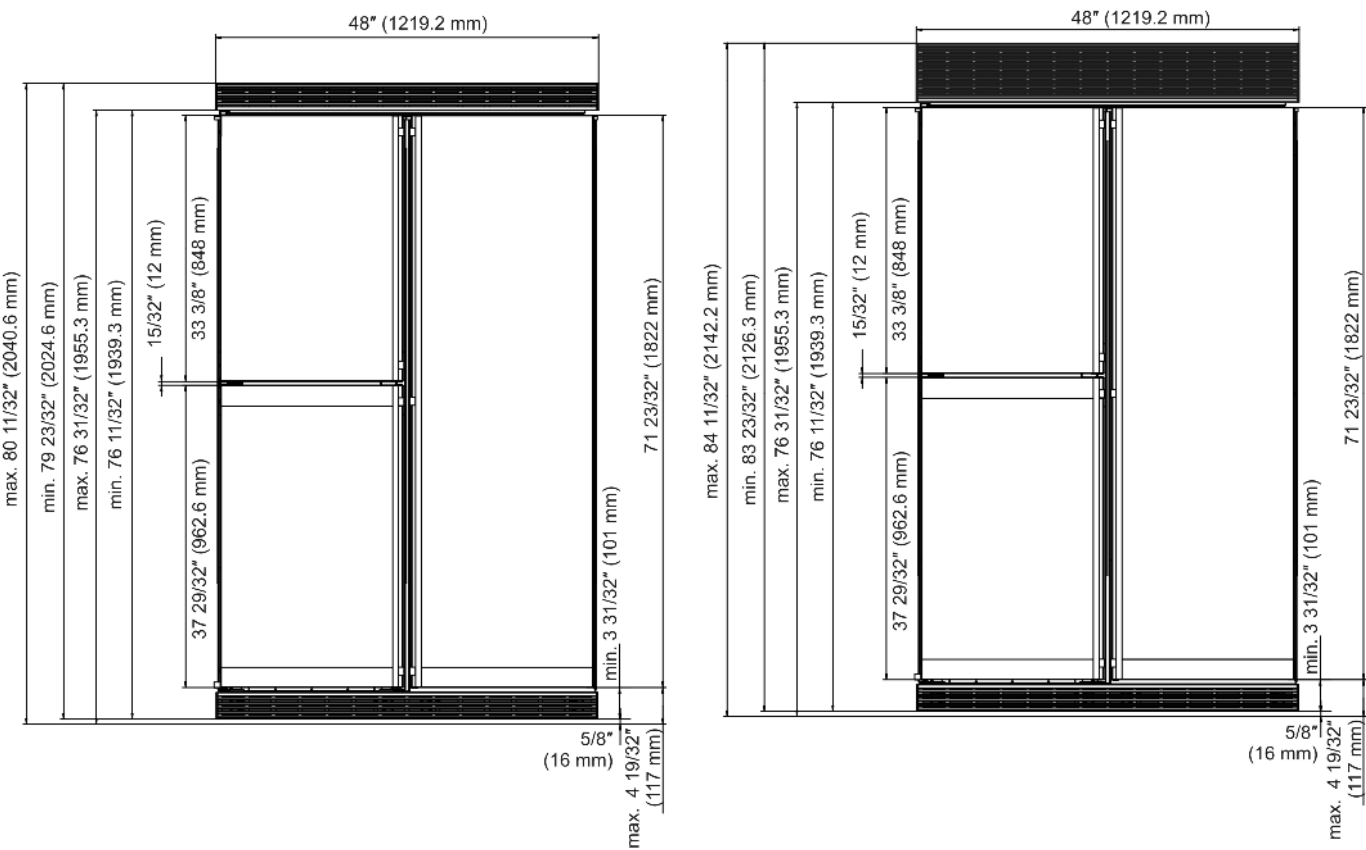
Fig. 3 Side-by-side installation: SBS 241 and SBS 246 with 80" or 84" ventilation grille
