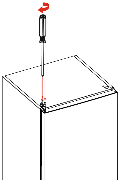
19. Secure the top hinge to the top of the unit.
