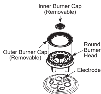
Multi-Ring Burner (on some models)
