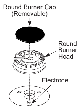
Round Burner
