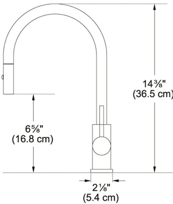
Technical Drawing
