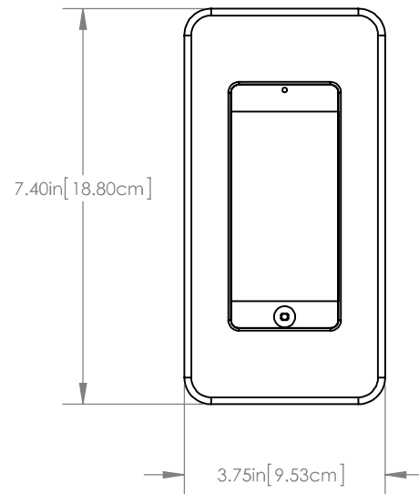
Front View with Bezel
