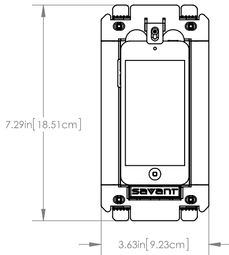
Front View without Bezel
