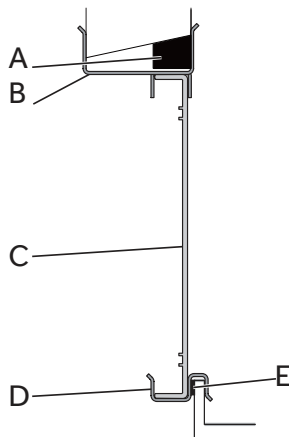
TYPICAL VINYL WINDOW INSTALLATION
