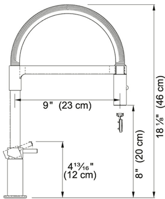
Technical Drawing
