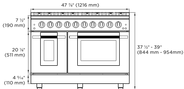
FRONT
