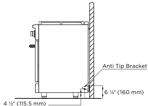
ANTI TIP
