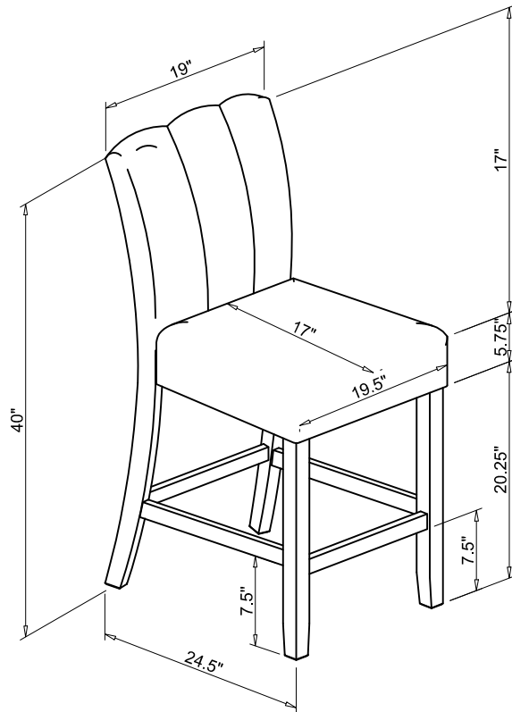
D06-BS Counter chair
