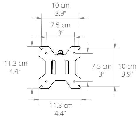
DETACHABLE MONITOR PLATE
