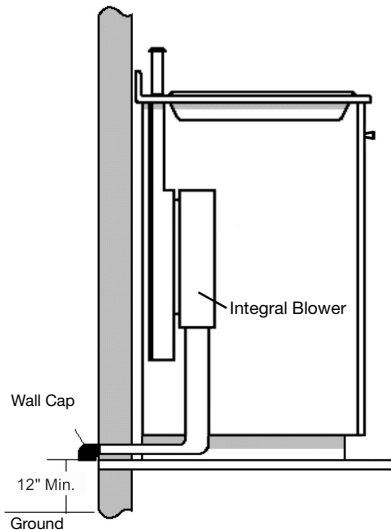
Integral Blower Through Wall Installation
