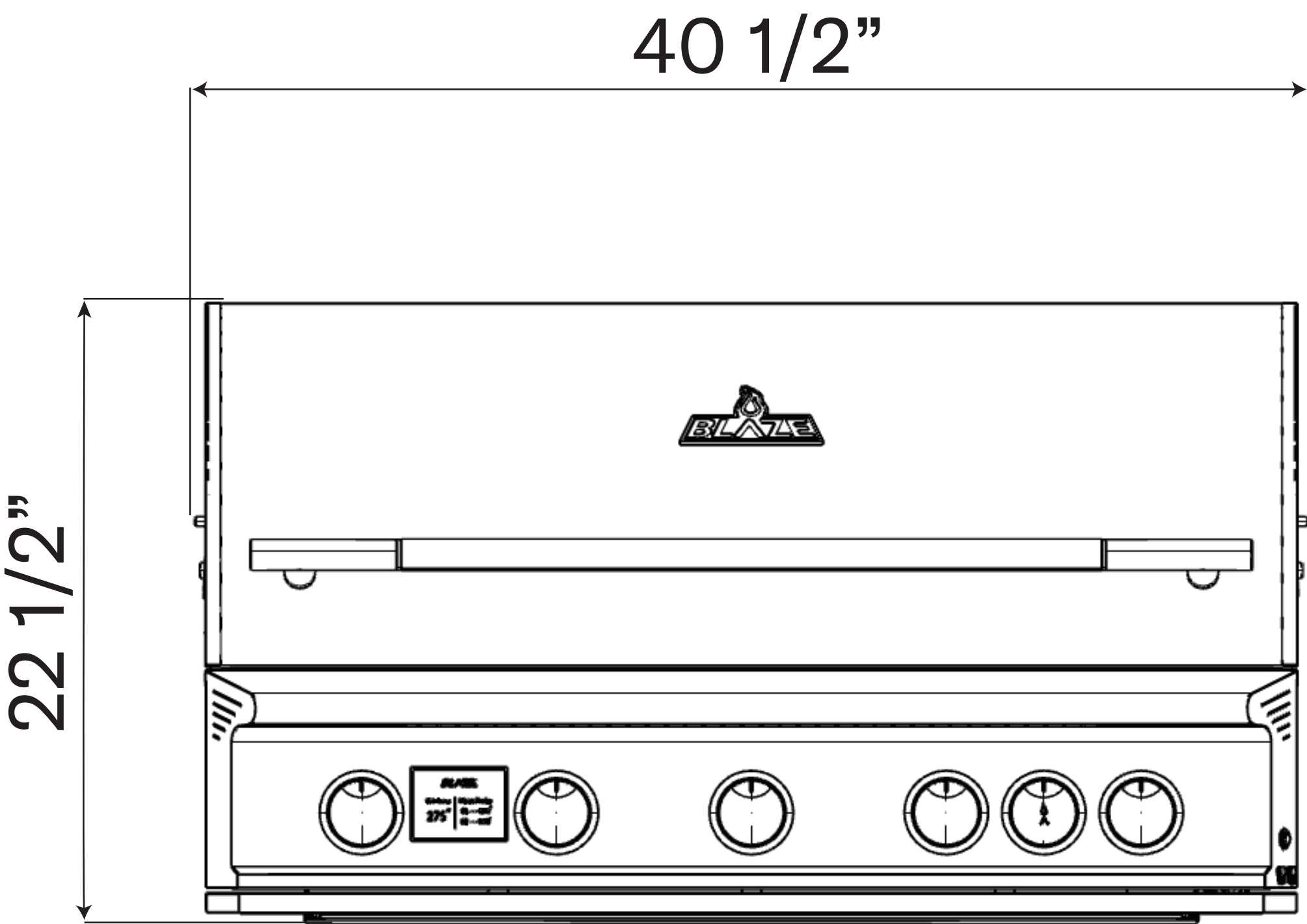
Front View
