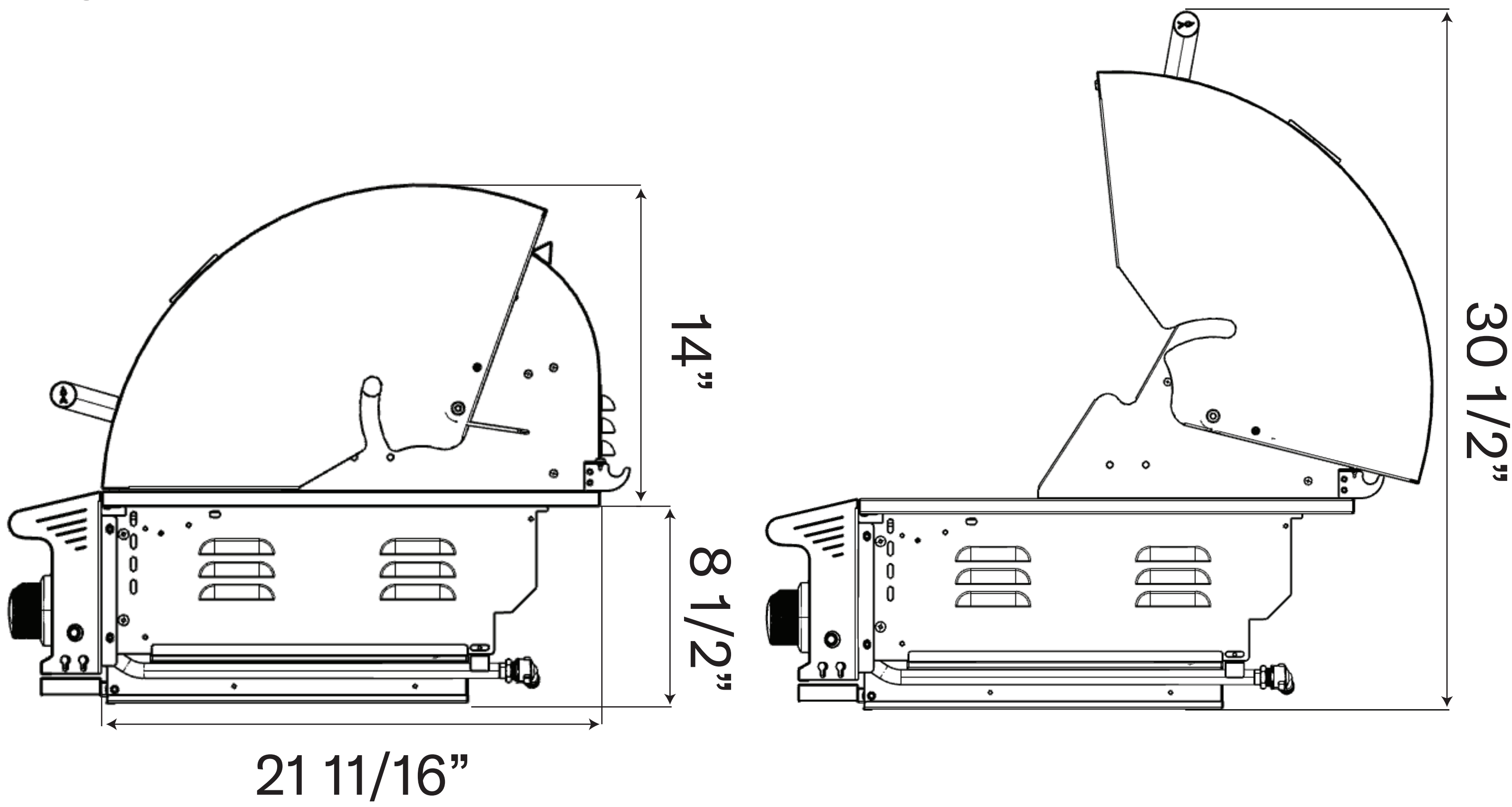
Side View
