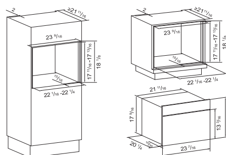
Flush Built-In
