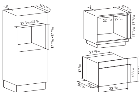
Standard Built-In
