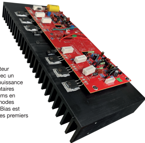
Triple push-pull transistors attached to a large radiator to ensure perfect heat dissipation.
