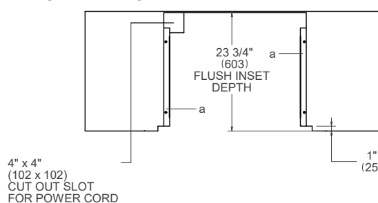
TOP VIEW – OVEN DETAIL
