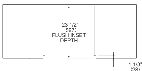
TOP VIEW – OVEN DETAIL
