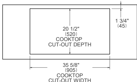
TOP VIEW – COOKTOP DETAIL
