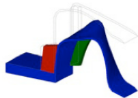
• FEA model showing the Z-Flex surround deformation as the cone moves backward.
