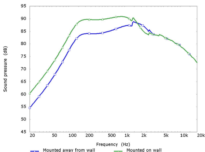
• Simulation showing the bass response boost wall effect.
