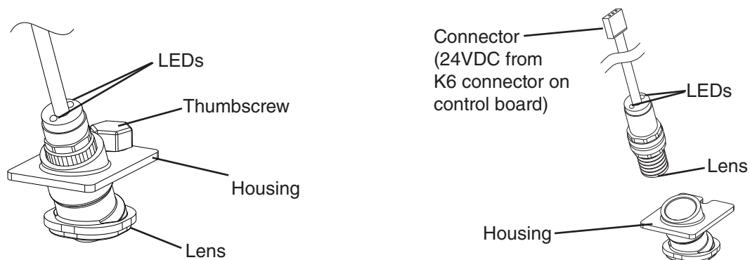
BC1 (infrared sensor)
