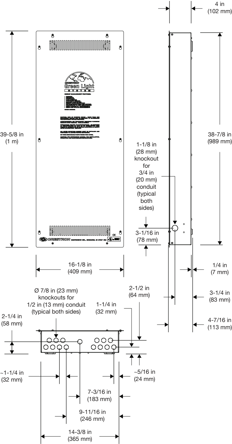
External Dimensions of DIN-EN-6X18 Rail Enclosures (Front, Side, and Bottom View)
