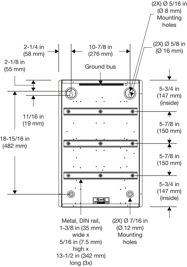
Internal Dimensions of DIN-EN-3X18 Rail Enclosures
