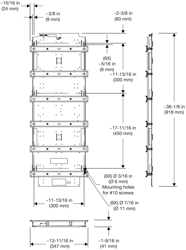
Dimensions of DIN-EN-6X18-MMP (Lay-In Panel)
