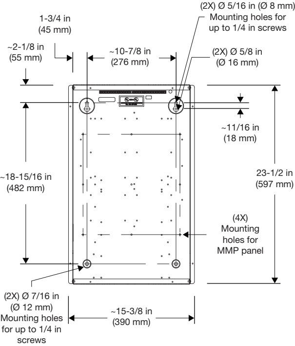
Dimensions of DIN-EN-3X18-MMP (Lay-In Panel)
