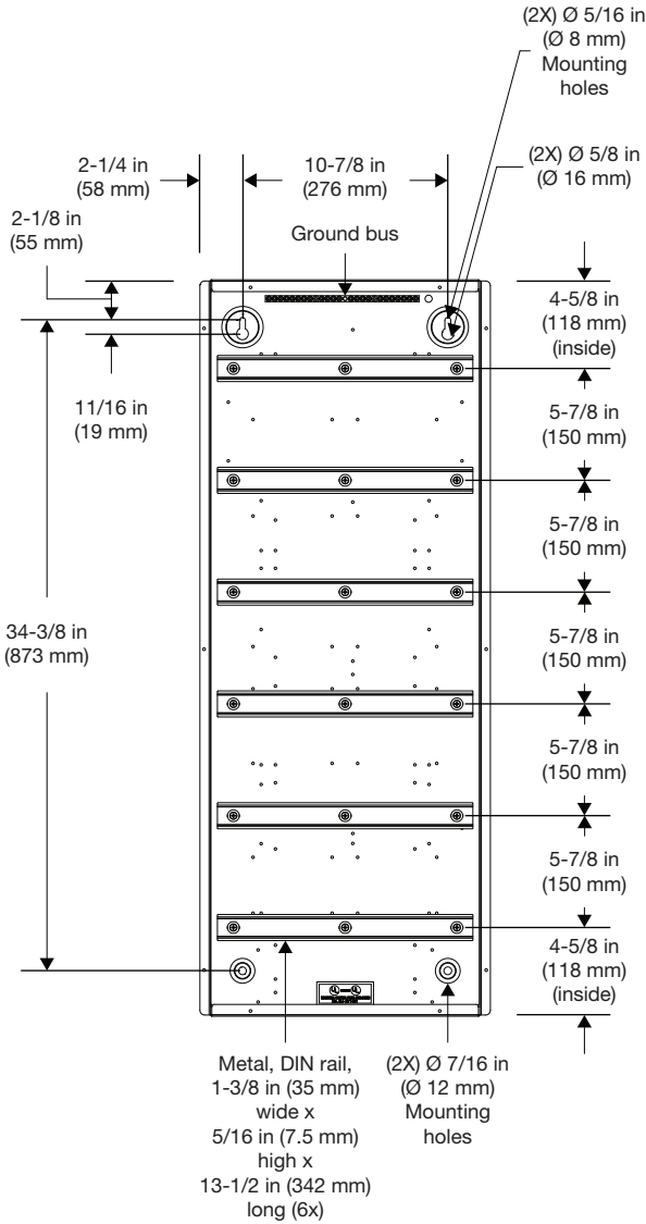
Internal Dimensions of DIN-EN-6X18 Rail Enclosures
