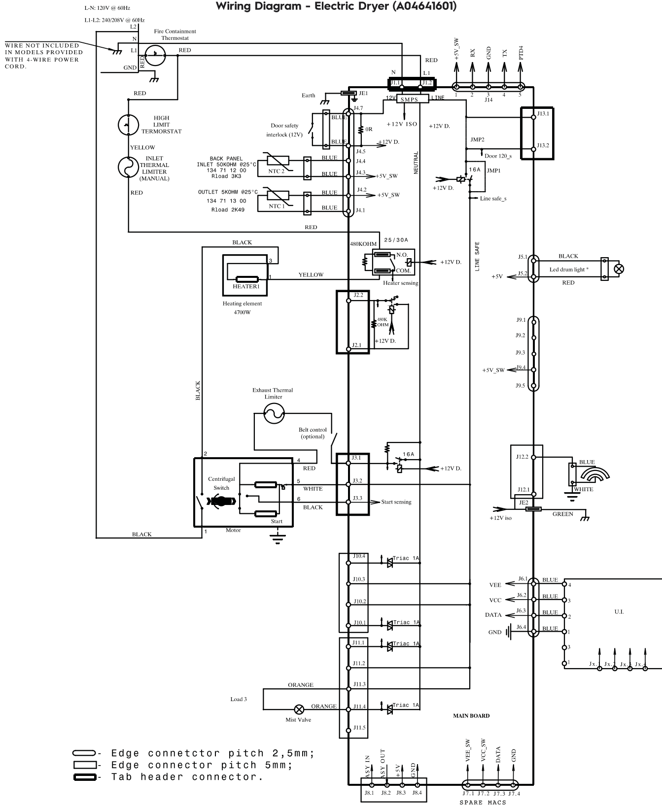
Wiring Diagram - Electric Dryer (A04641601)
