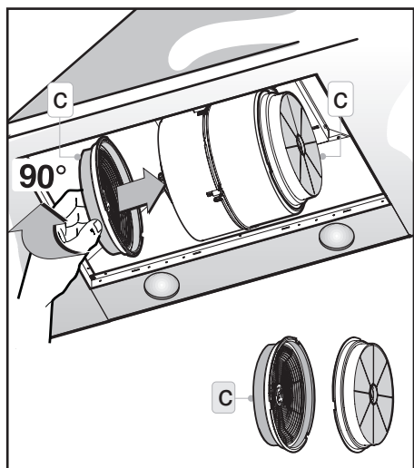
Fig.9: The filters C must be applied to the suction unit inside the hood, centering them inside of it and turning them 90° until they snap into place.
