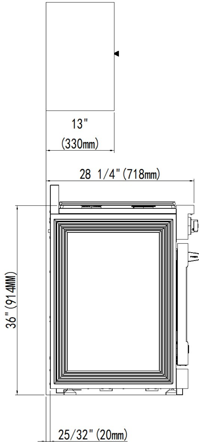
Side View
