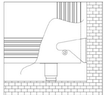
Anti-tip device for RSG36P/PB
