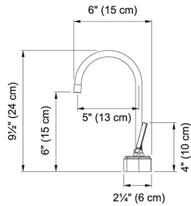
Technical Drawing
