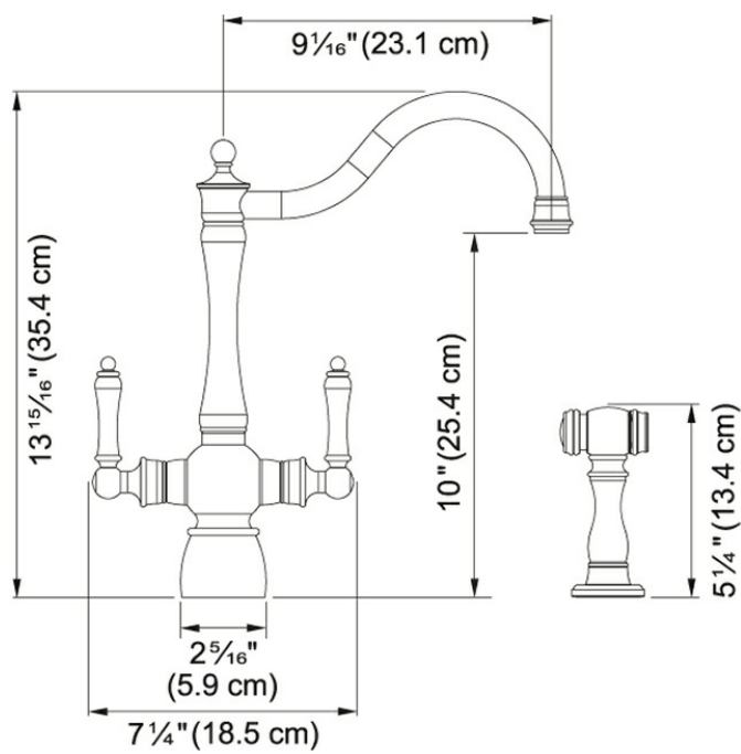
Technical Drawing
