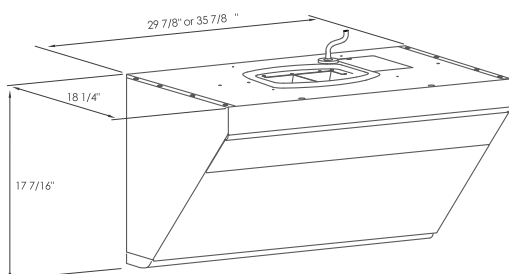
▲ Product Dimensions
