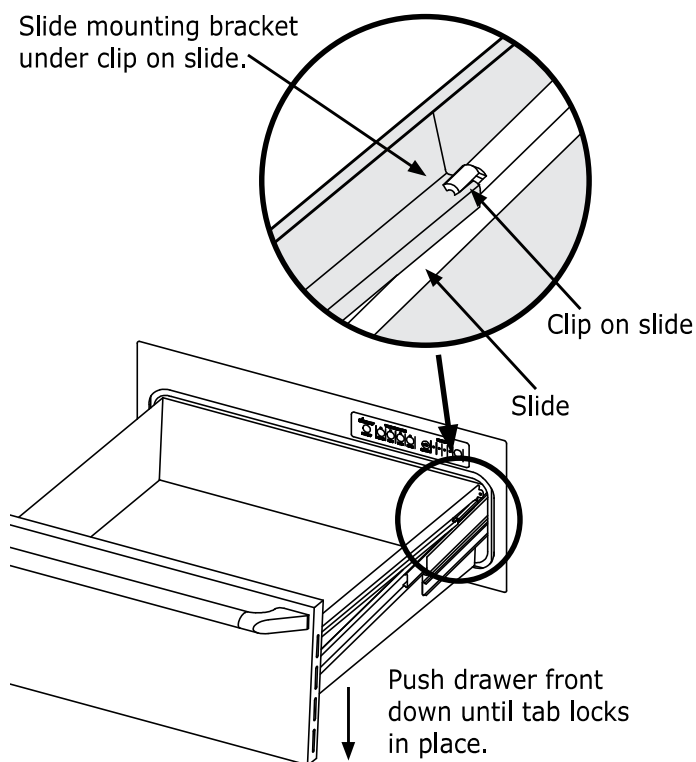
Drawer Installation
