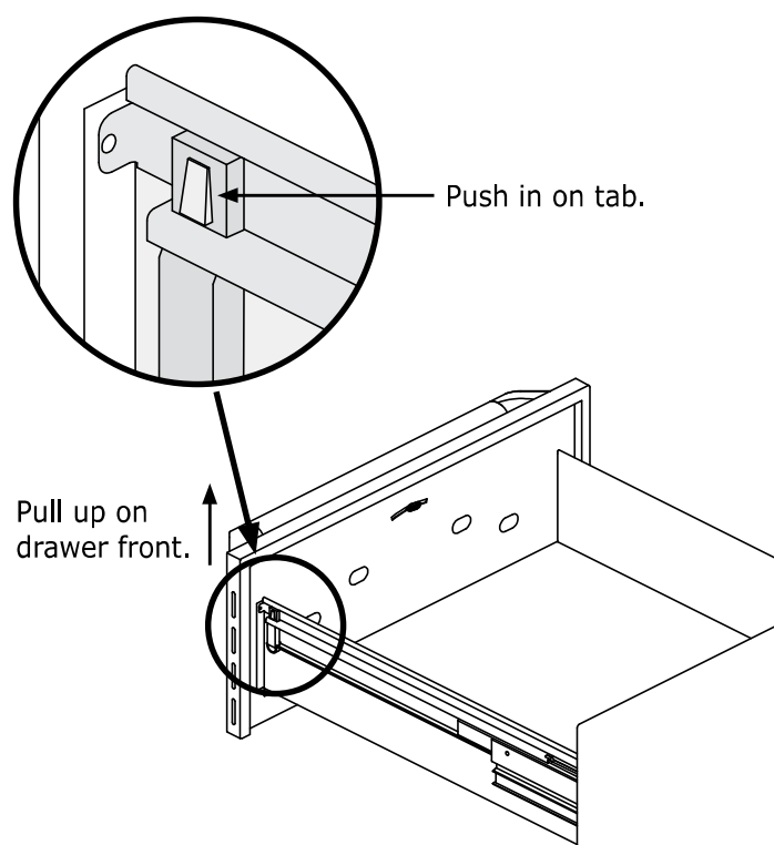
Drawer Removal
