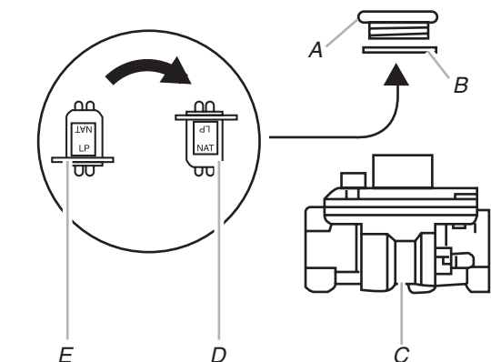
A. Access cap B. Gasket C. Gas pressure regulator D. NAT position E. LP position
