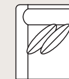
4712 LAF One Arm Chair 4713 RAF One Arm Chair Overall: H 37 W 34 D 39 Seating: H 17 W 26 D 23 Seat Height: 20 Arm Height: 24 Pillows: 2 P21
