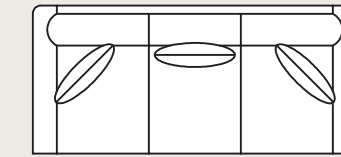
4775 Sofa Overall: H 37 W 86 D 39 Seating: H 17 W 70 D 23 Seat Height: 20 Arm Height: 24 Pillows: 2 P21, 1 P2415
