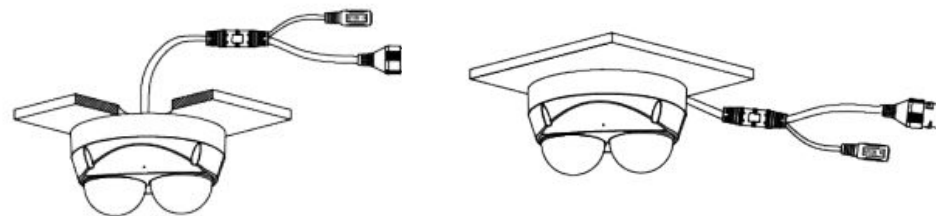
Mounting surface exit vs Side exit
