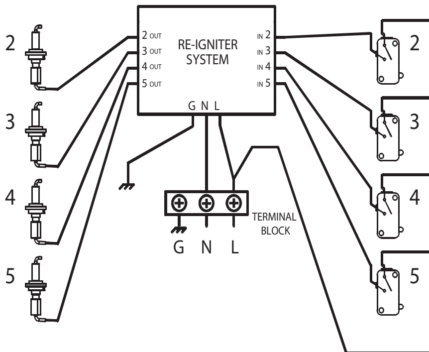
Figure 15. Wiring diagram (4 zones)
