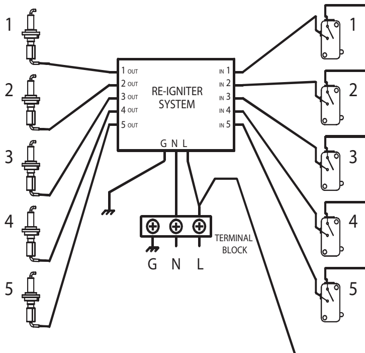
Figure 16. Wiring diagram (5 zones)
