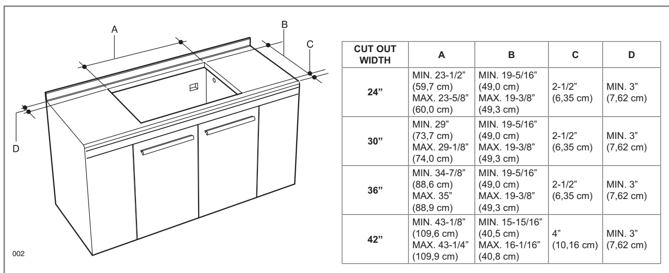
Figure 2. Coutout dimensions
