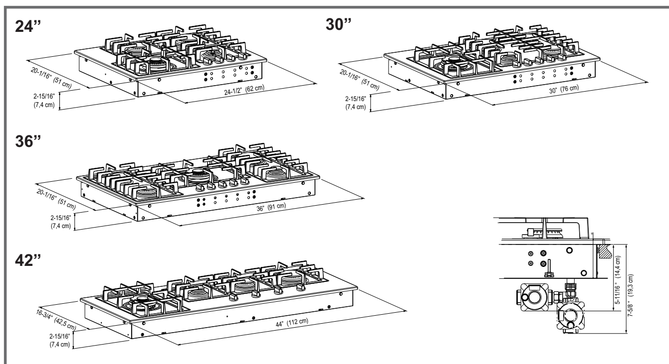
Figure 1. Product dimensions
