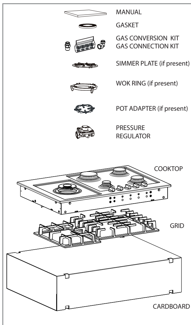
Figure 6. Parts
