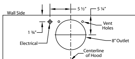
B200 Dual Blower (Top View)
