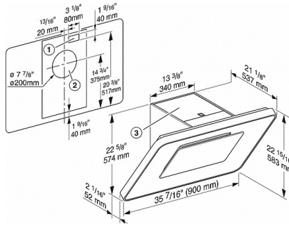
DA 6996 W (Installation drawing) - USA
