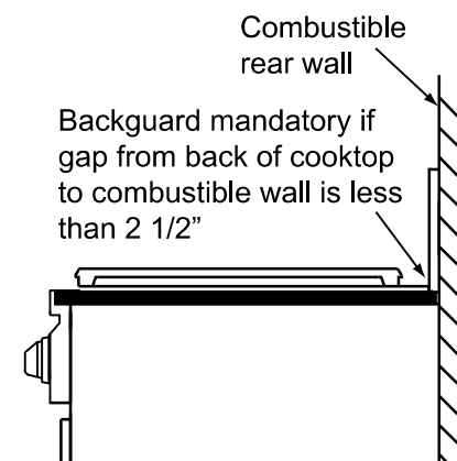
SIDE VIEW WITHOUT BACKGUARD
