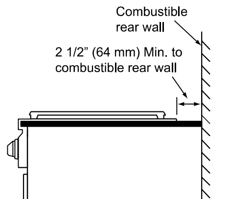
SIDE VIEW WITHOUT BACKGUARD
