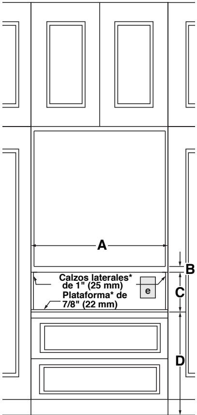
VISTA FRONTAL
