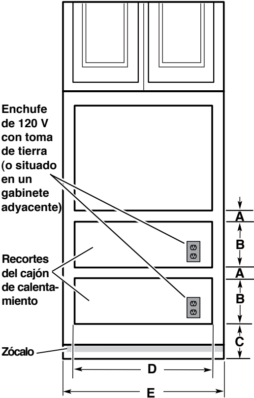
VISTA FRONTAL
