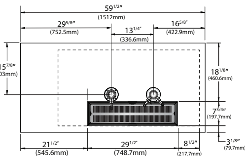
DD59(-S) Plan View
