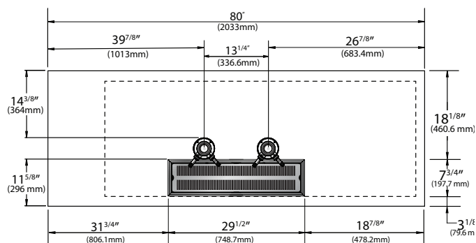
DD80(-S) Plan View
