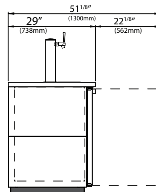
All Models Side View
