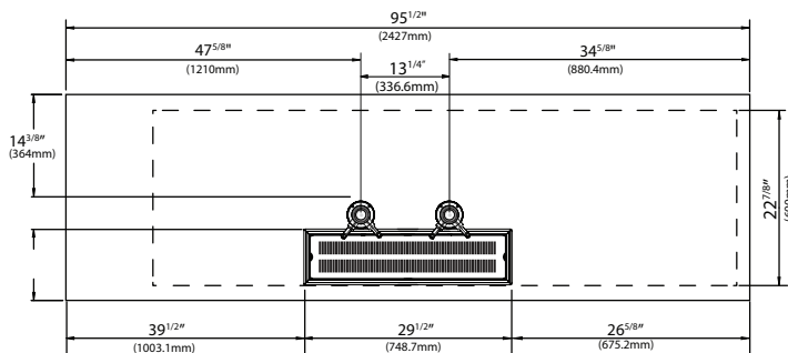
DD95(-S) Plan View
