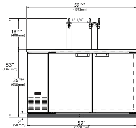
DD59(-S) Front View
