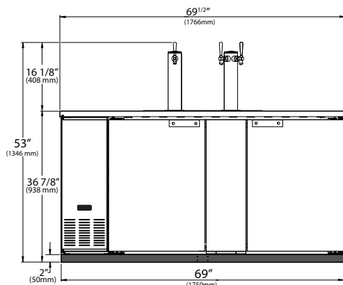
DD69(-S) Front View
