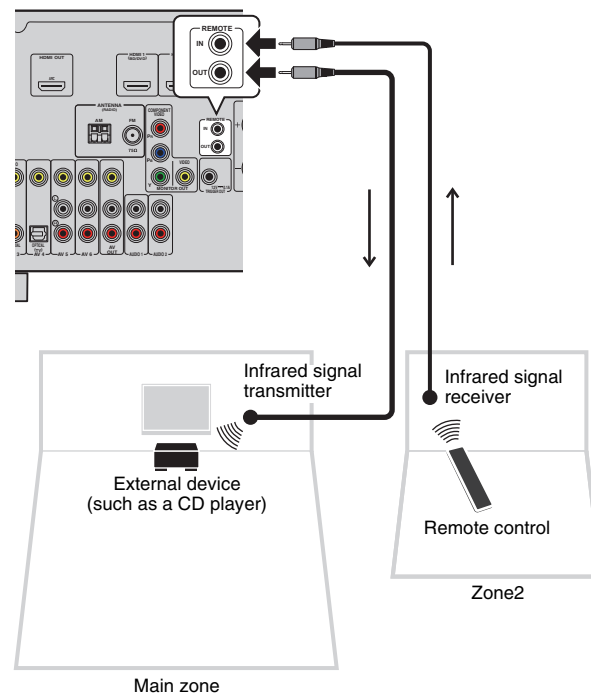
The unit (rear) REMOTE IN/OUT jacks
