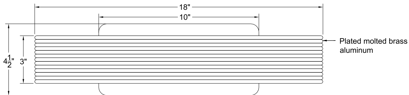
SIDE VIEW
