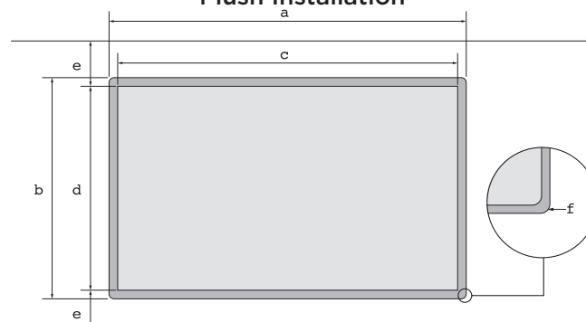
Flush Installation
