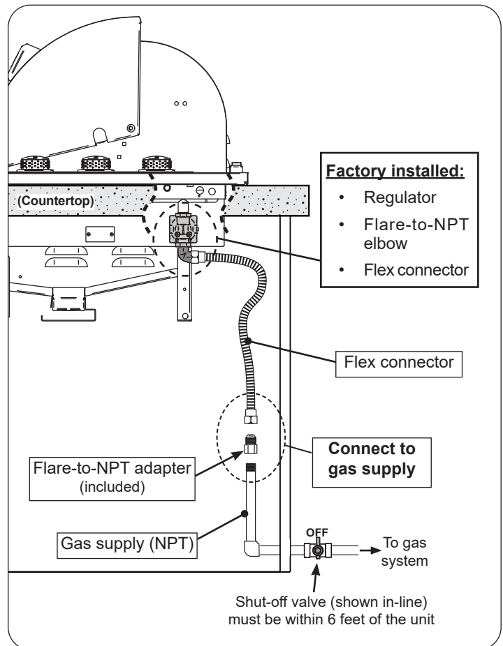
Fig. 31-1 Household L.P. & Nat. gas diagram
