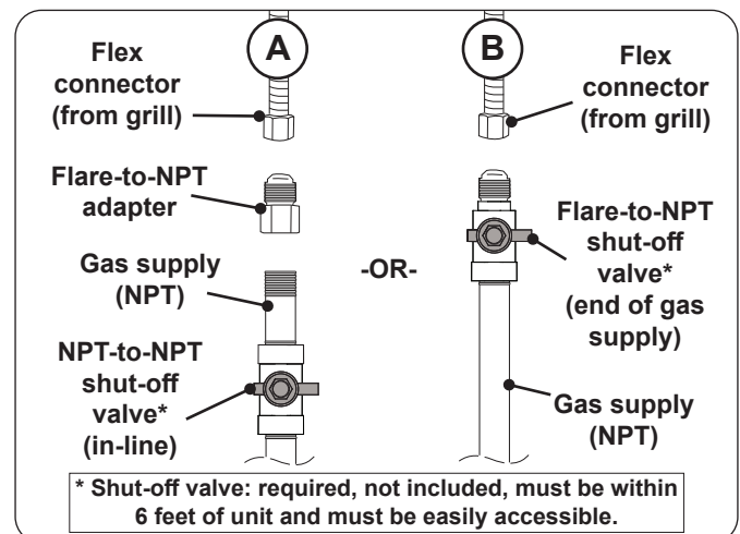
Fig. 31-2 Connecting to a gas line
