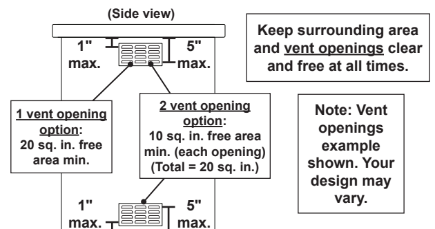
Fig. 12-3 Natural gas ventilation detail
