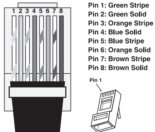
Figure 2: RJ-45 Audio Connector
