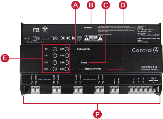
Figure 1: Front view
