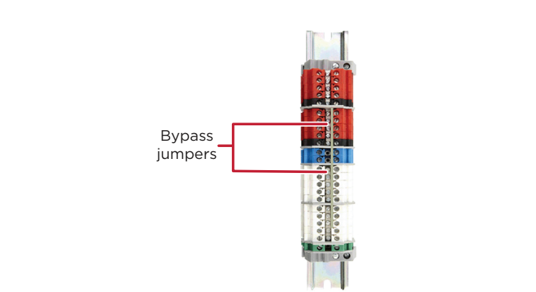
Figure 2: Terminal block bypass jumpers
