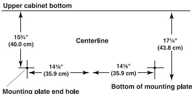
Mounting plate end hole
