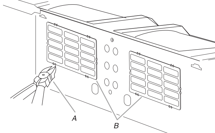
A. Diagonal wire cutting pliers B. Louvered damper vent covers
