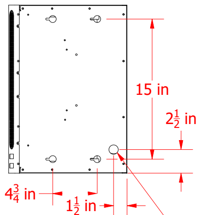
TOP VIEW (CLOSED)
