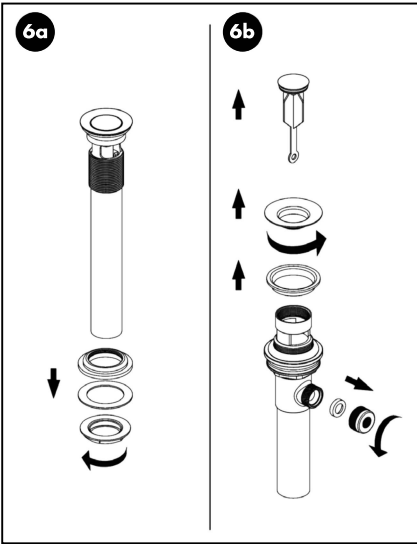
Remove the washers, nut, and flange from the pop-up drain.
